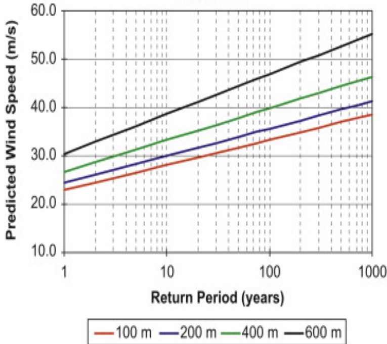
Predicted Wind Speeds by height from NAMNARR
